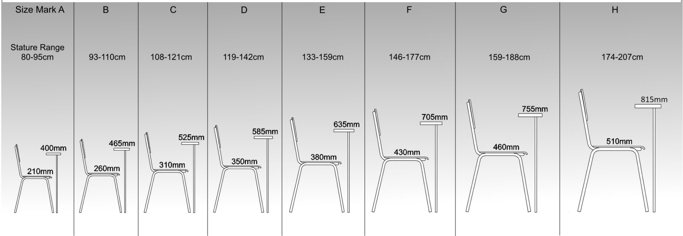
CHAIR HEIGHTS ± 10mm, TABLE HEIGHTS ± 15mm
