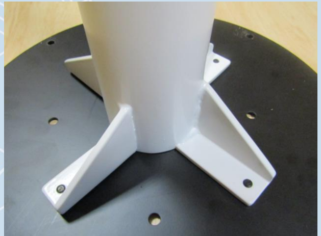
4 bolts - Table top disc to pedestal
